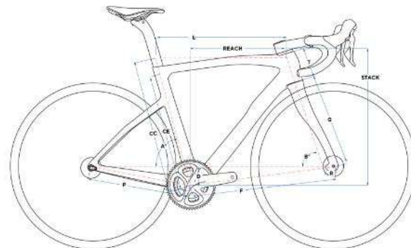
CE: SEAT TUBE CENTER - END, CC: SEAT TUBE CENTER - CENTER, L: TOP TUBE CENTER - CENTER, A[°]: SEAT TUBE ANGLE, B[°]: HEADTUBE ANGLE, P: CHAINSTAY, T: HEADTUBE, D: BB DROP, R: FORK RAKE, G: FORK HEIGHT, REACH, STACK
